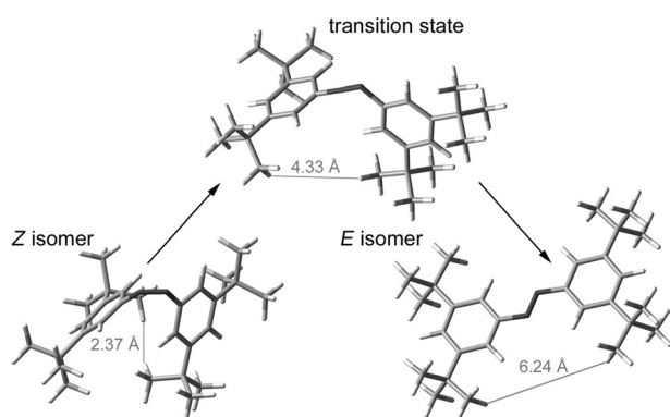
Scheme 2. Geometry optimization of the Z and the E isomers and the transition state of the thermal isomerization of tert -butylazobenzene 4 [B3LYP-D3/6-311G(d,p)].
