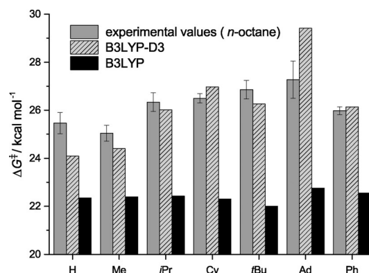
Figure 2. Experiment versus computation with a 6-311G(d,p) basis set (55 °C).
