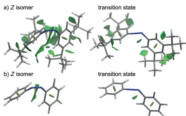
Figure 3. NCI analysis of the optimized [B3LYP-D3/6-311G(d,p)] Z isomers and transition states of tert -butyl derivative 4 (a) and azobenzene 3 (b), visualized using VMD. [33]
