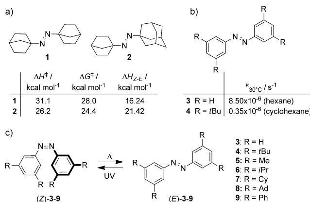
Scheme 1. a) Kinetic and thermodynamic data for the thermal Z to E isomerization of two aliphatic azo compounds in mesitylene. b) k values of two meta -substituted azobenzenes for the thermal Z to E isomerization. c) The thermal Z to E isomerization of seven differently substituted azobenzenes investigated in this study (Ad = adamantyl, Cy = cyclohexyl).
