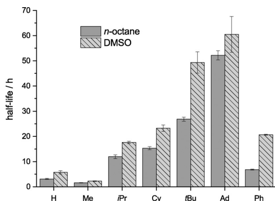
Figure 1. Half-lives of azobenzenes 3–9 measured in n -octane and DMSO at 53 °C.
